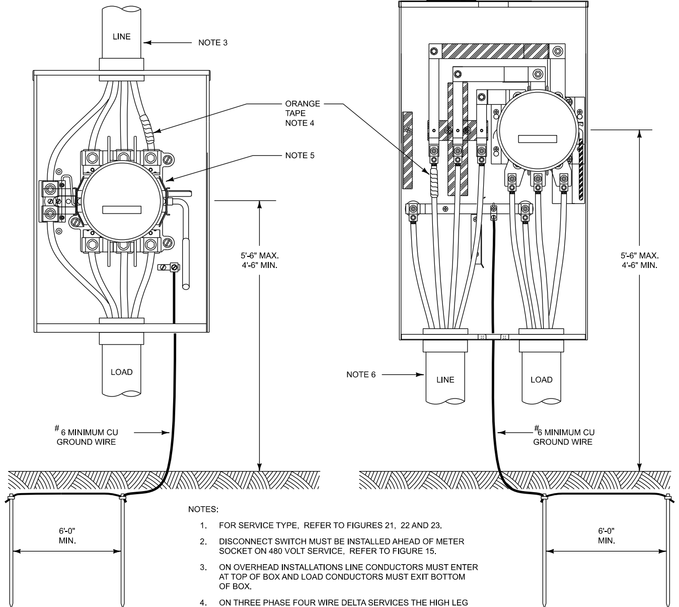
THREE PHASE 4 WIRE 320 AMP SOCKET METER BOX WITH BY-PASS SWITCH NOTES 1 AND 2
