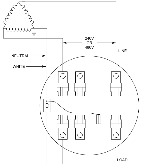
3 WIRE 240 OR 480 VOLT THREE PHASE SELF CONTAINED 7 TERMINAL SOCKET
