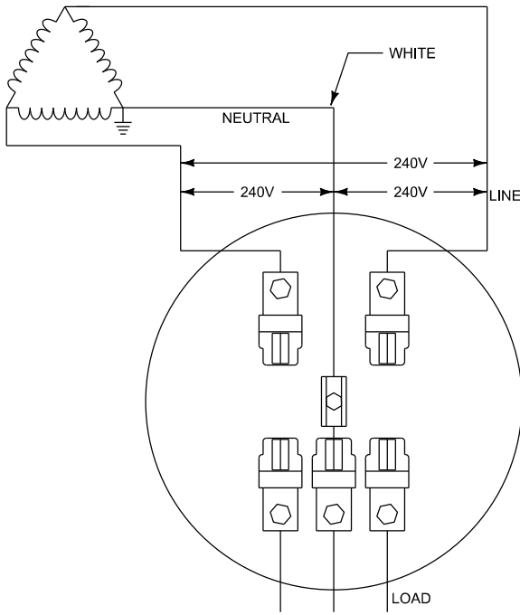
3 WIRE 240 VOLT THREE PHASE SELF CONTAINED CENTER PHASE DISCONNECT
