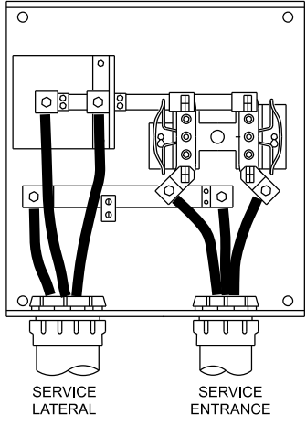
DETAIL "B" METER BASE
