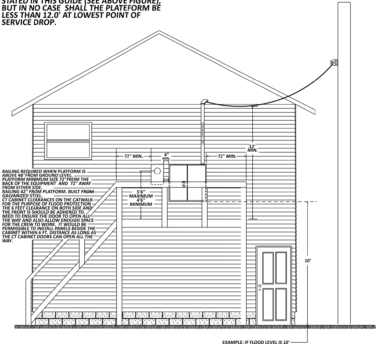
TYPICAL OVERHEAD CT CABINET AND METER EQUIPMENT CATWALK INSTALLATION WALL MOUNT ABOVE FLOOD LEVEL WITH PLATFORM
