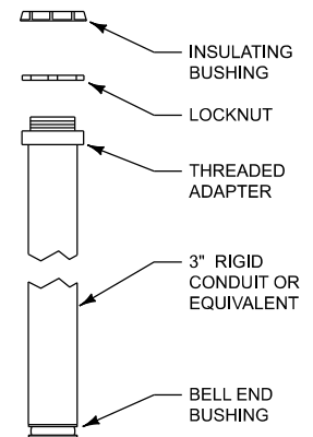
DETAIL "B" RISER ASSEMBLY
