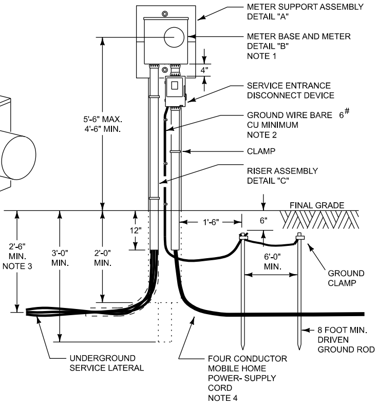
DETAIL "A" METER SUPPORT ASSEMBLY
