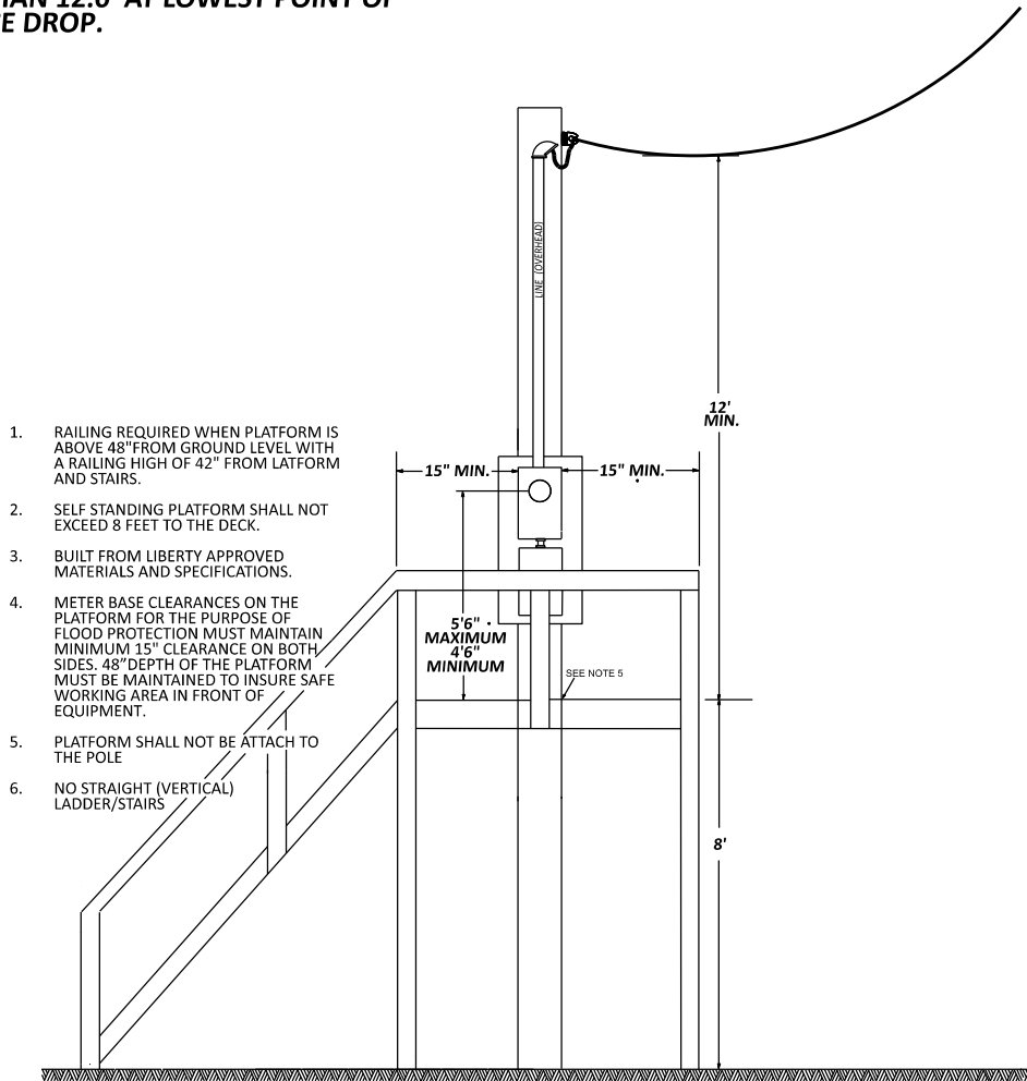
TYPICAL OVERHEAD METER EQUIPMENT SELF-STANDING PLATFORM INSTALLATION POLE MOUNT ABOVE FLOOD LEVEL
