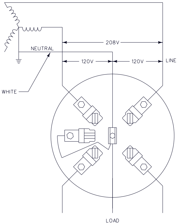
3 WIRE NETWORK 120/208 VOLT SINGLE PHASE SELF CONTAINED
