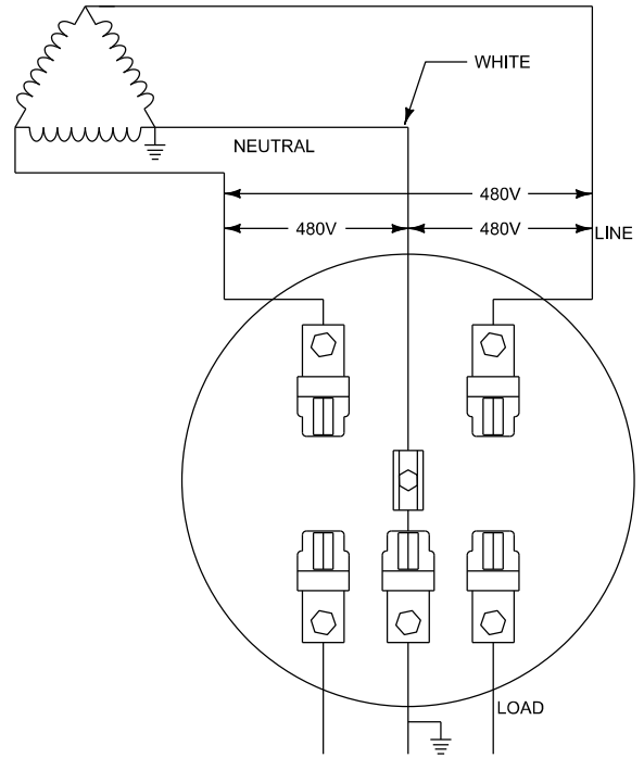
3 WIRE 480 VOLT THREE PHASE SELF CONTAINED CENTER PHASE DISCONNECT
